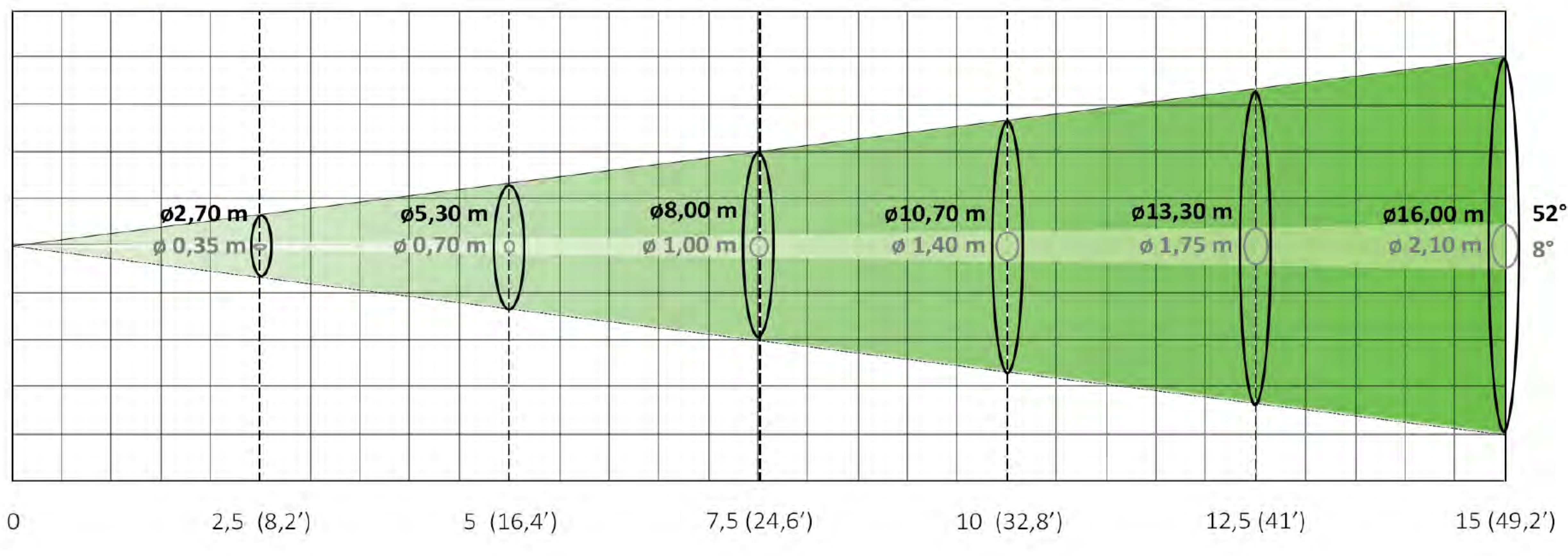
Illuminance distribution DIVUM 50K
