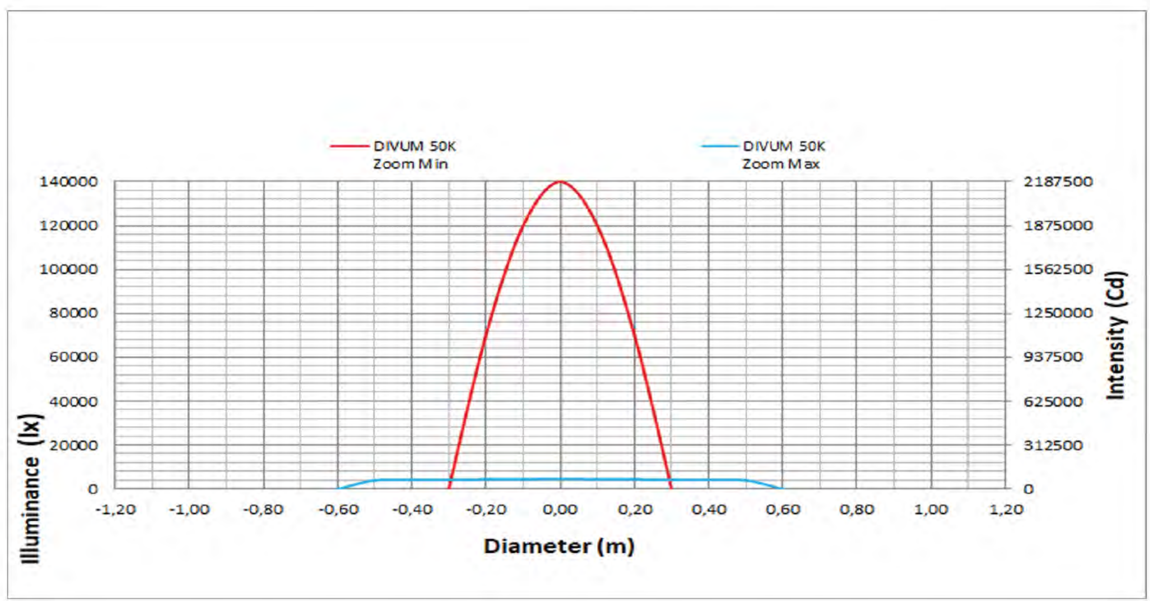
Illuminance distribution DIVUM 50K
