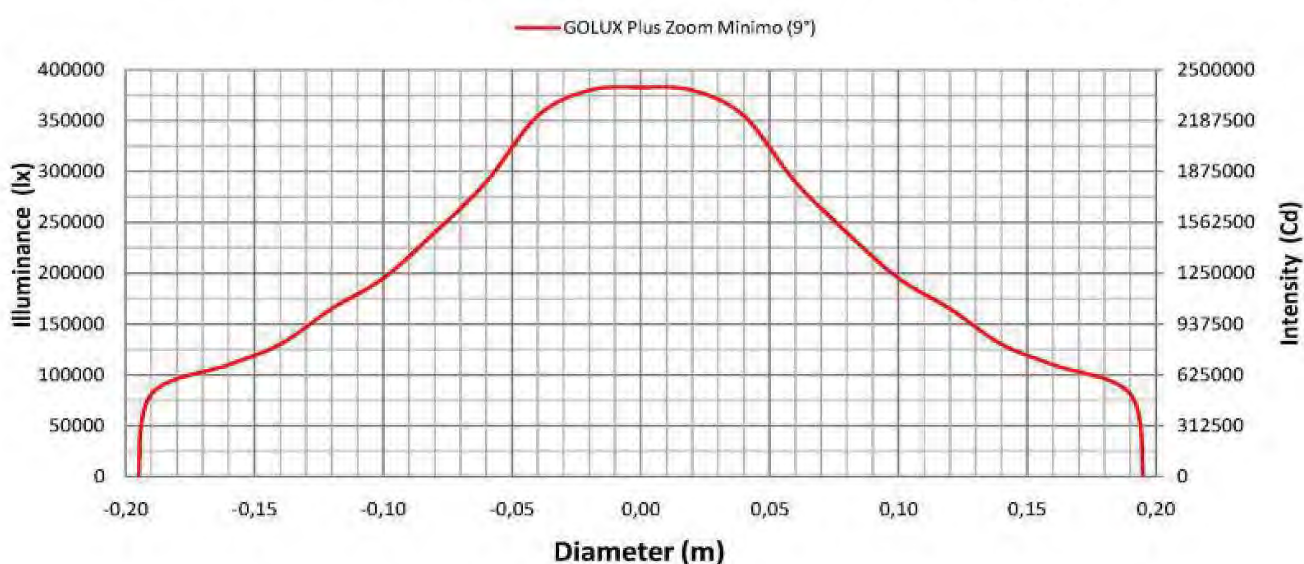
Illuminance distribution GOLUX Plus - Zoom minimo (Distance = 2,5 m)
